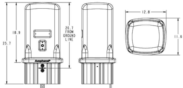
Dimensional Views All dimensions are in inches.
