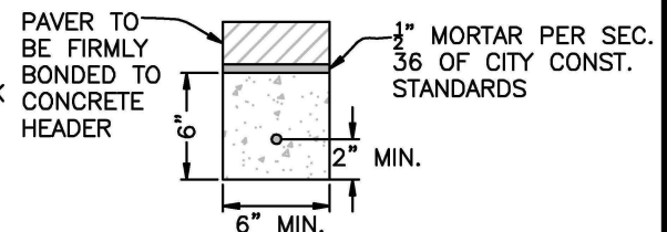
ALTERNATE HEADER CURB DETAIL
